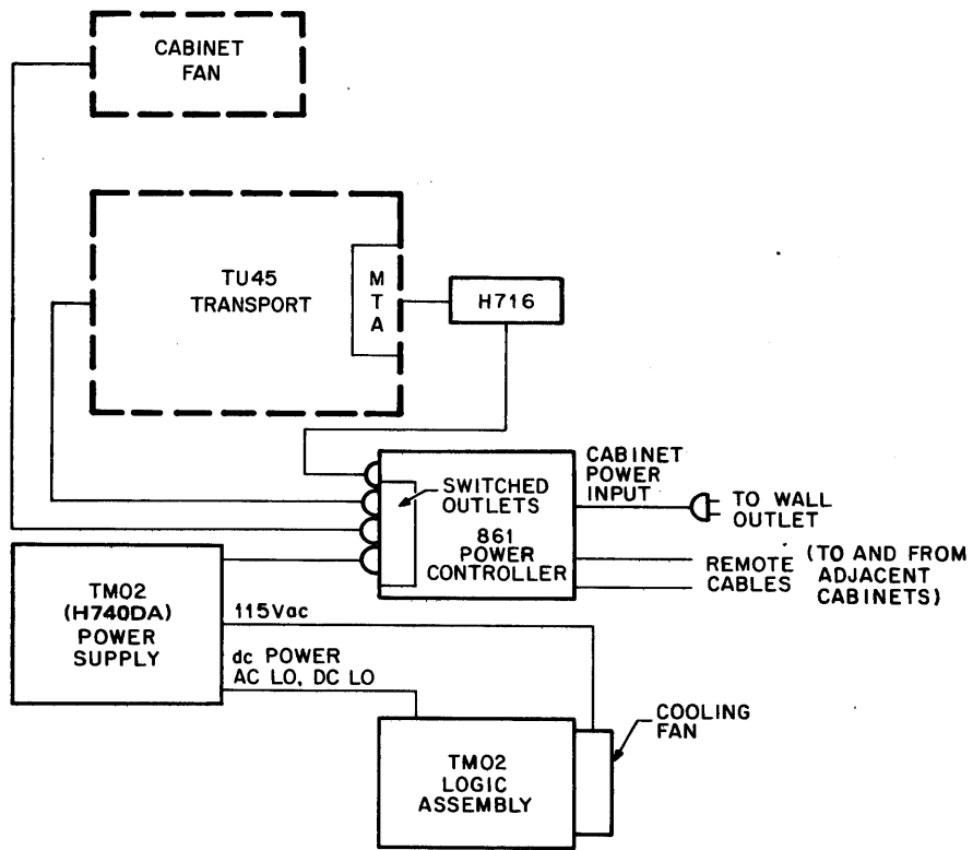
Figure 1-11 TU45/TM02 Power System
