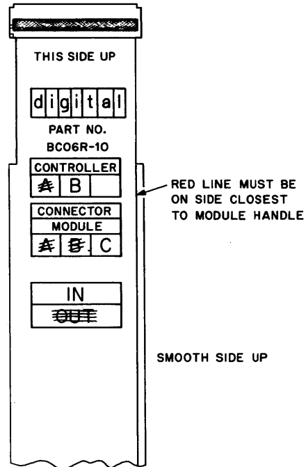
Figure 2-5 Marked-Up Massbus Cable
