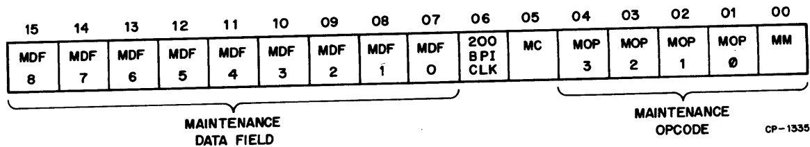
Figure 3-13 Maintenance Register Bit Usage
