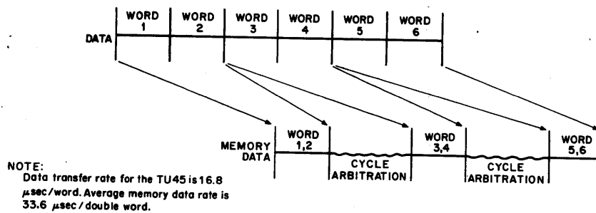
Figure 1-3 Read Data Transfer Sequence
