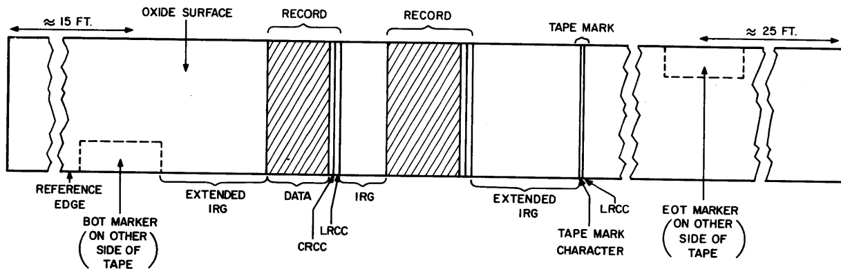
Figure 1-8 NRZI Format (Nine-Channel)
