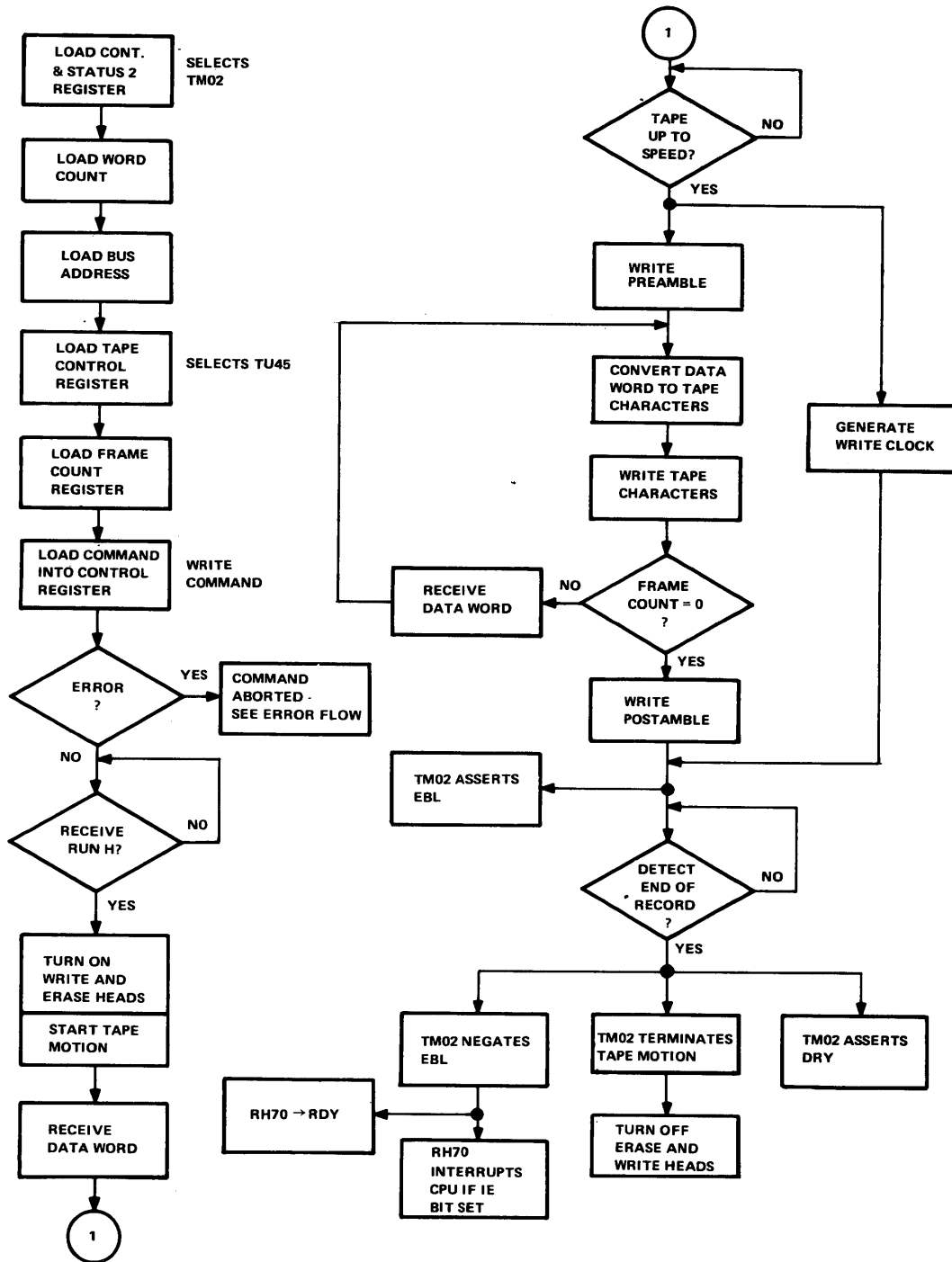
Figure 4-6 PE Data Write Operation Flowchart
