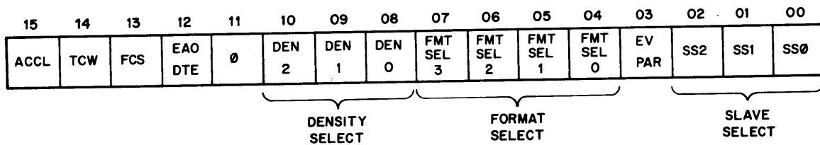
Figure 3-16 Tape Control Register Bit Usage
