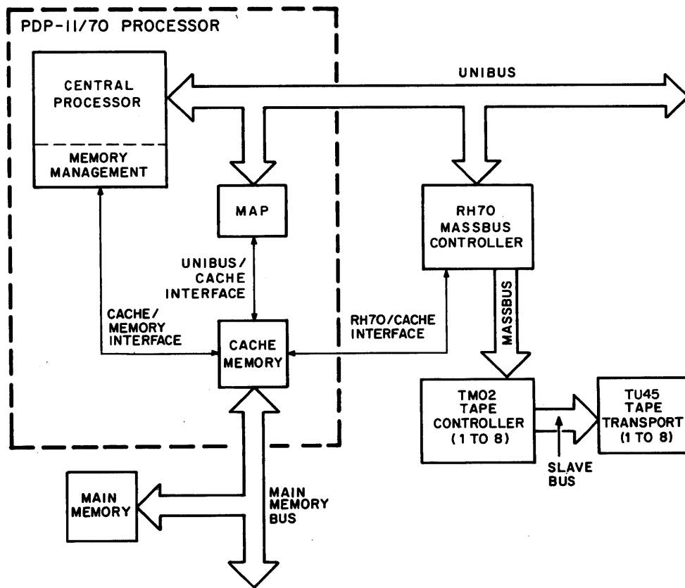
Figure 1-1 TWU45 Simplified System Diagram
