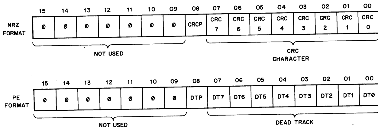
Figure 3-11 Check Character Register Format
