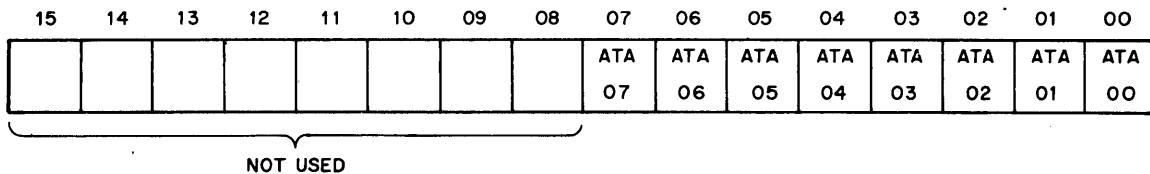
Figure 3-10 Attention Summary Register Bit Usage
