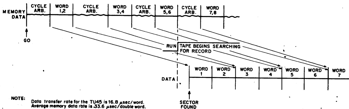
Figure 1-4 Write Data Transfer Sequence
