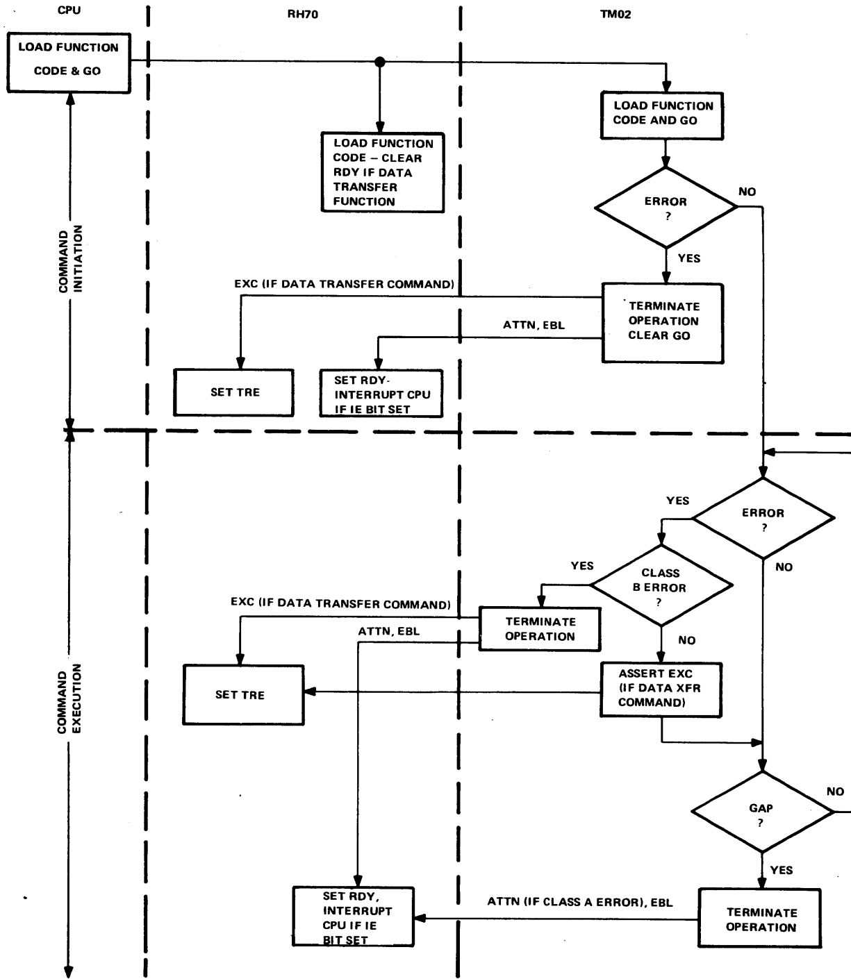
Figure 1-5 RH70 Error Termination
