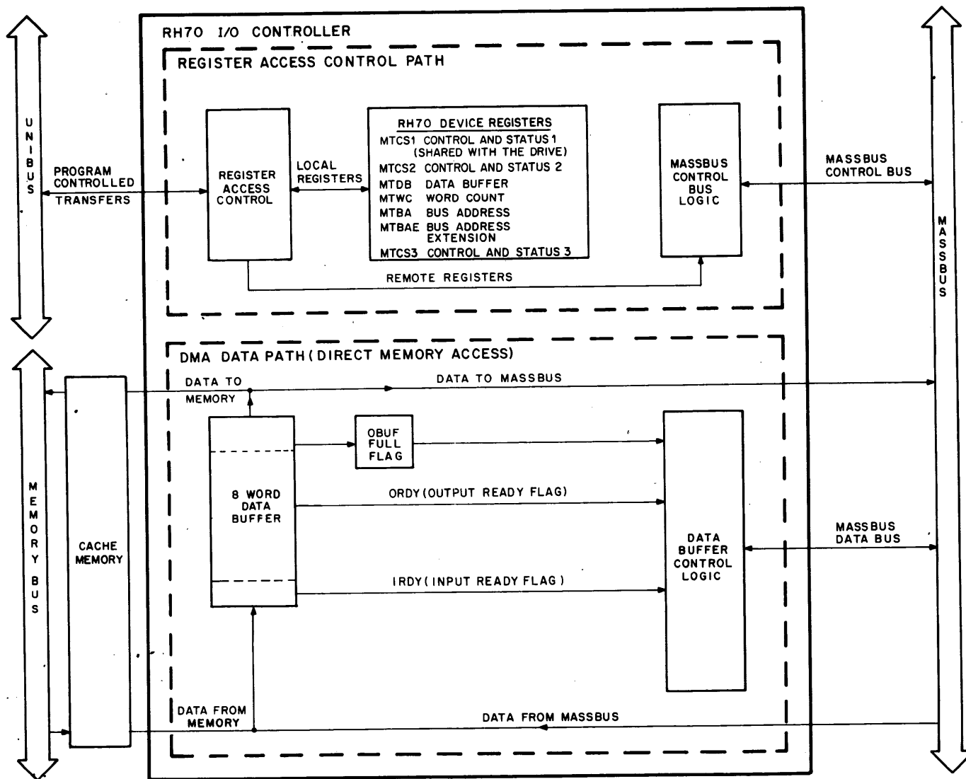
Figure 1-2 RH70 Simplified Data Path Diagram
